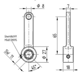
Change Lever 65
