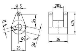
Change Lever 24
